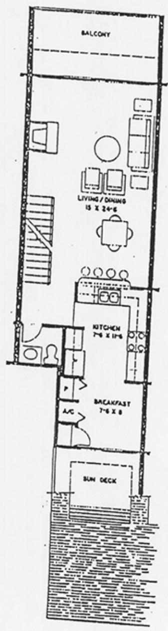
SECOND FLOOR
